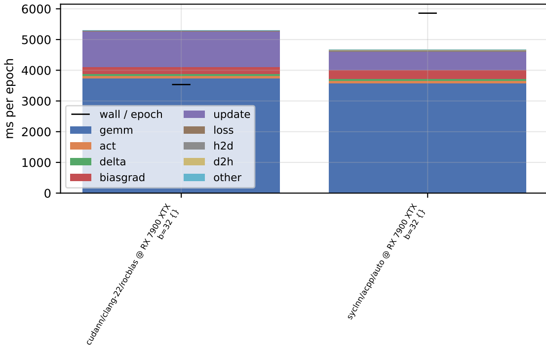
per-phase device time - sweep-w1024-d4-b32 (double, train)
