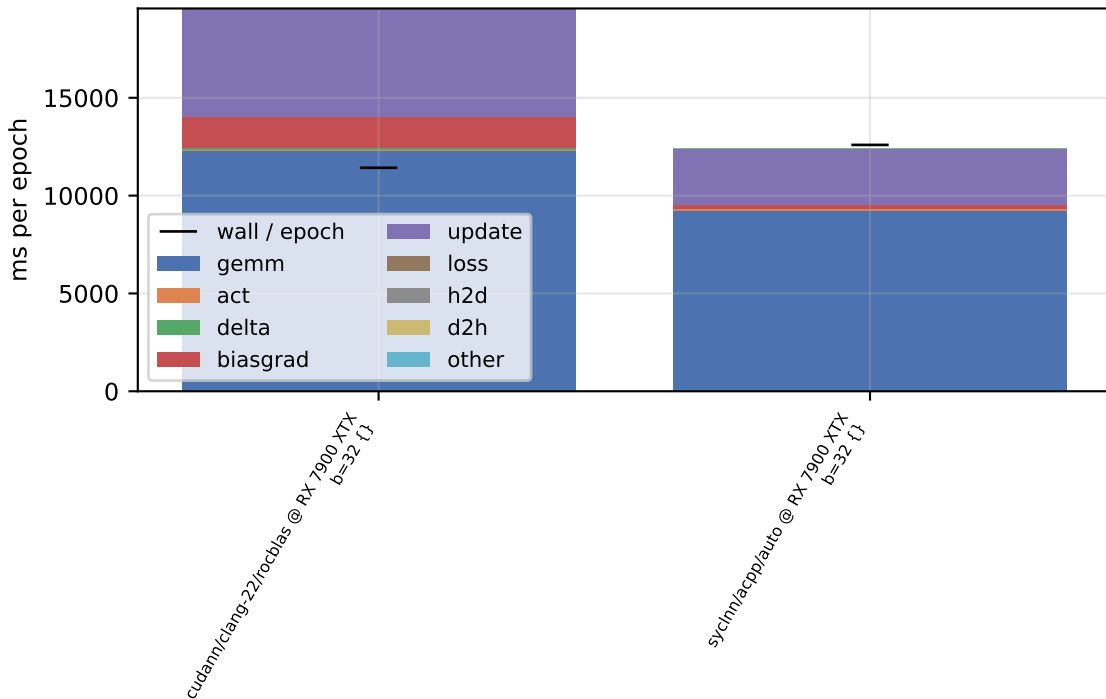
per-phase device time - sweep-w4096-d2-b32 (double, train)
