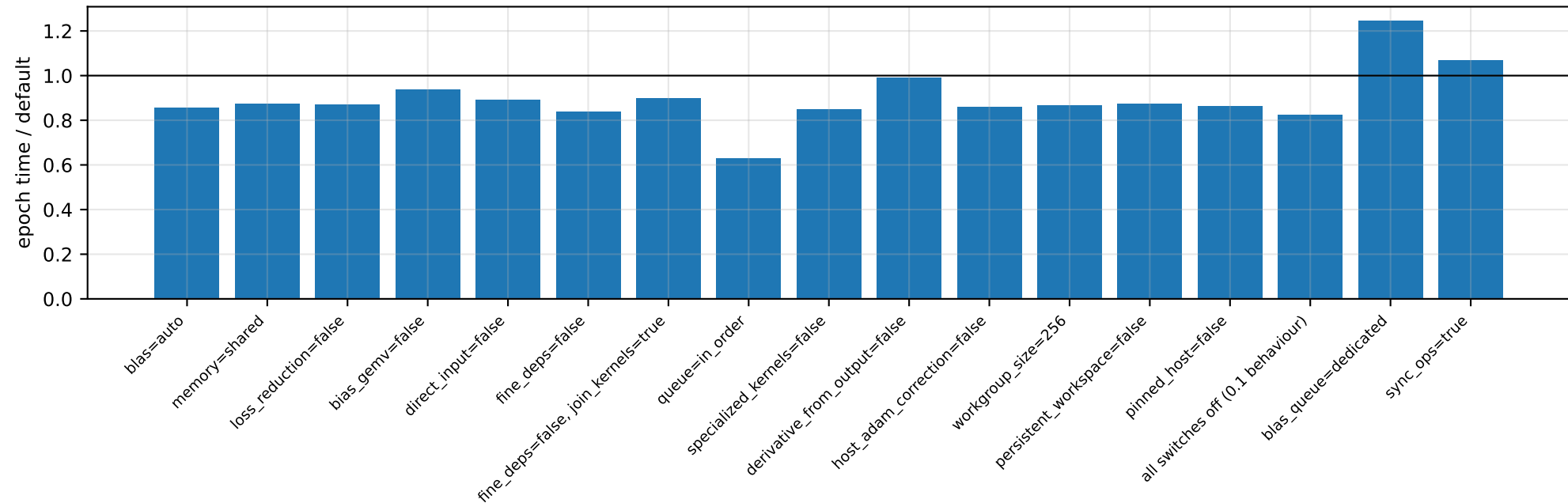
syclnn ablations - monk (float, b=40) on RX 7900 XTX
