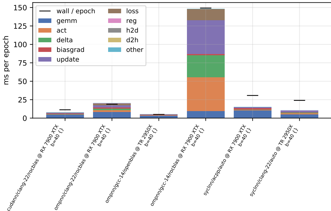
per-phase device time - cup (double, train)
