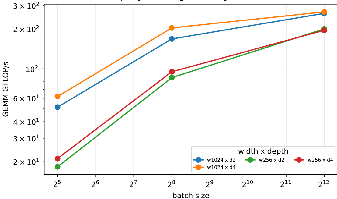
W4 sweep - syclnn/clang-22/auto @ TR 2950X (float)
