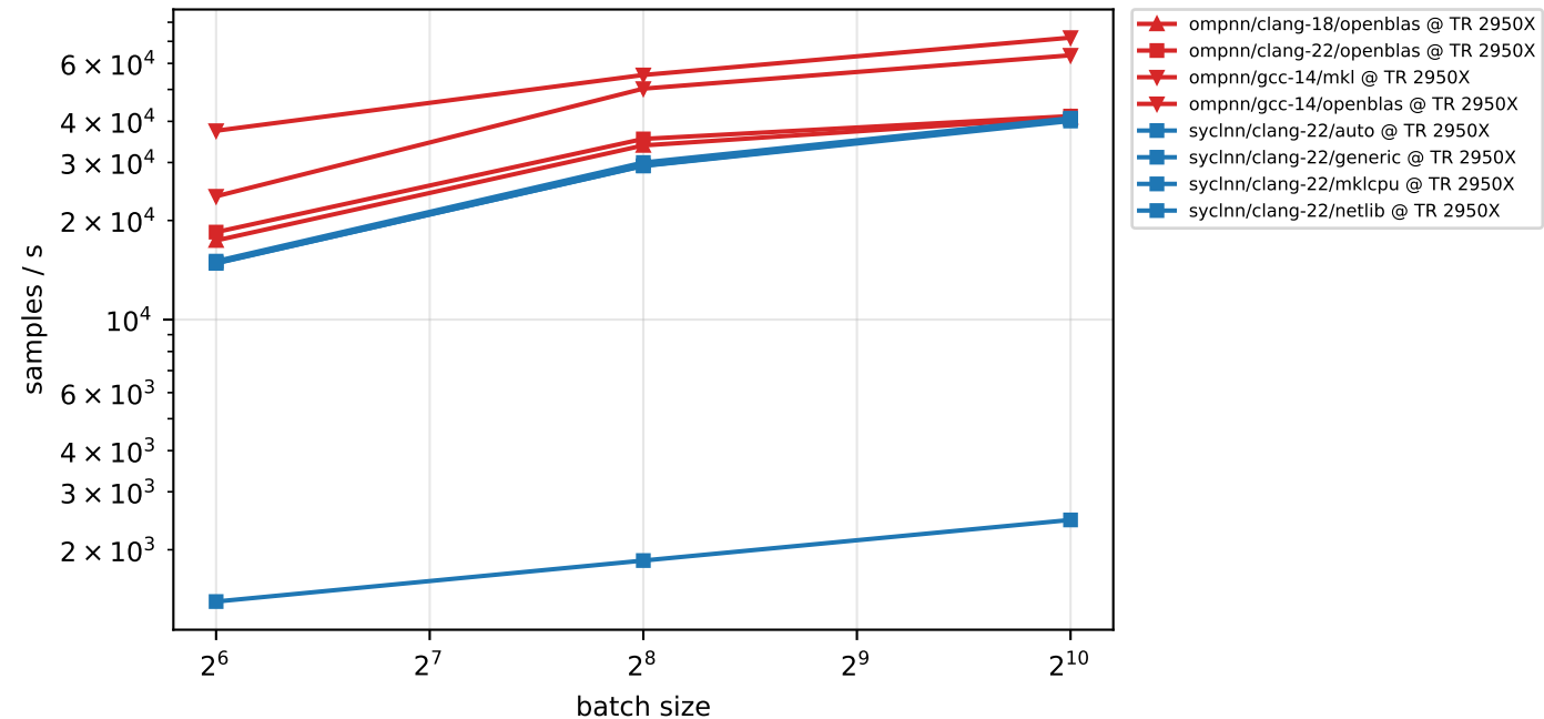
training throughput - mnist-512-256 (double, cpu)
