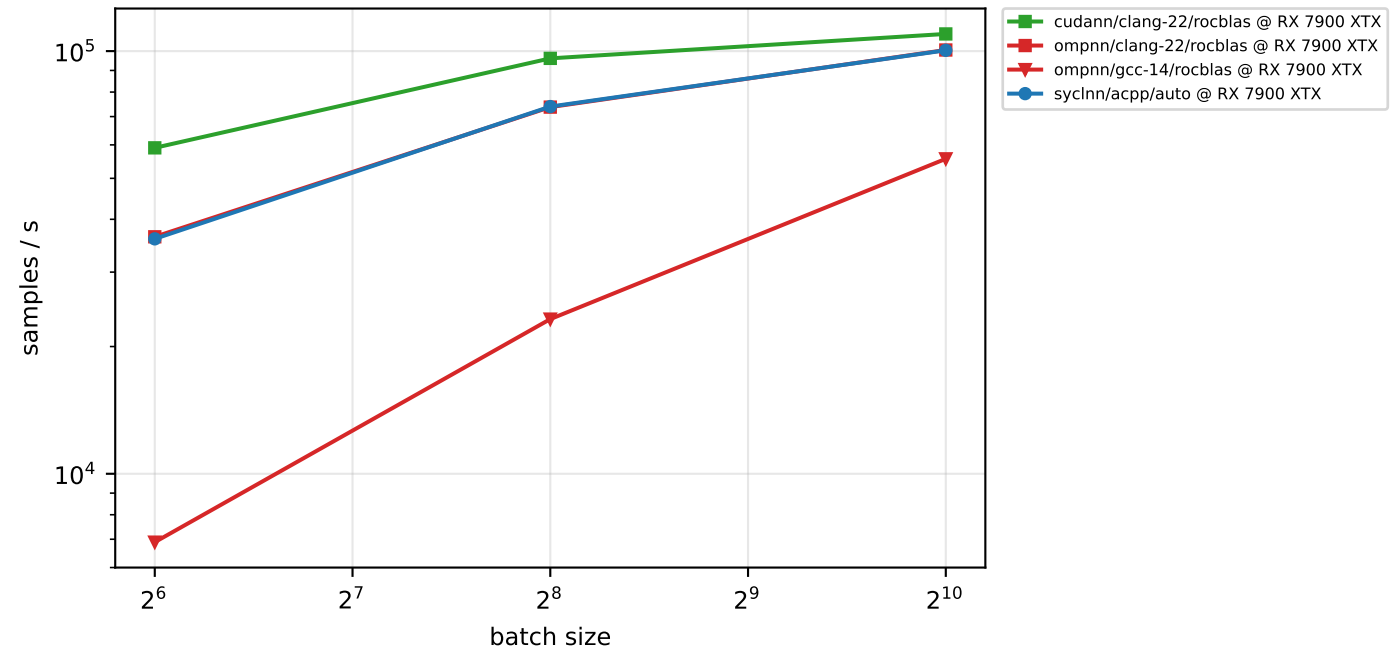
training throughput - mnist (double, gpu)
