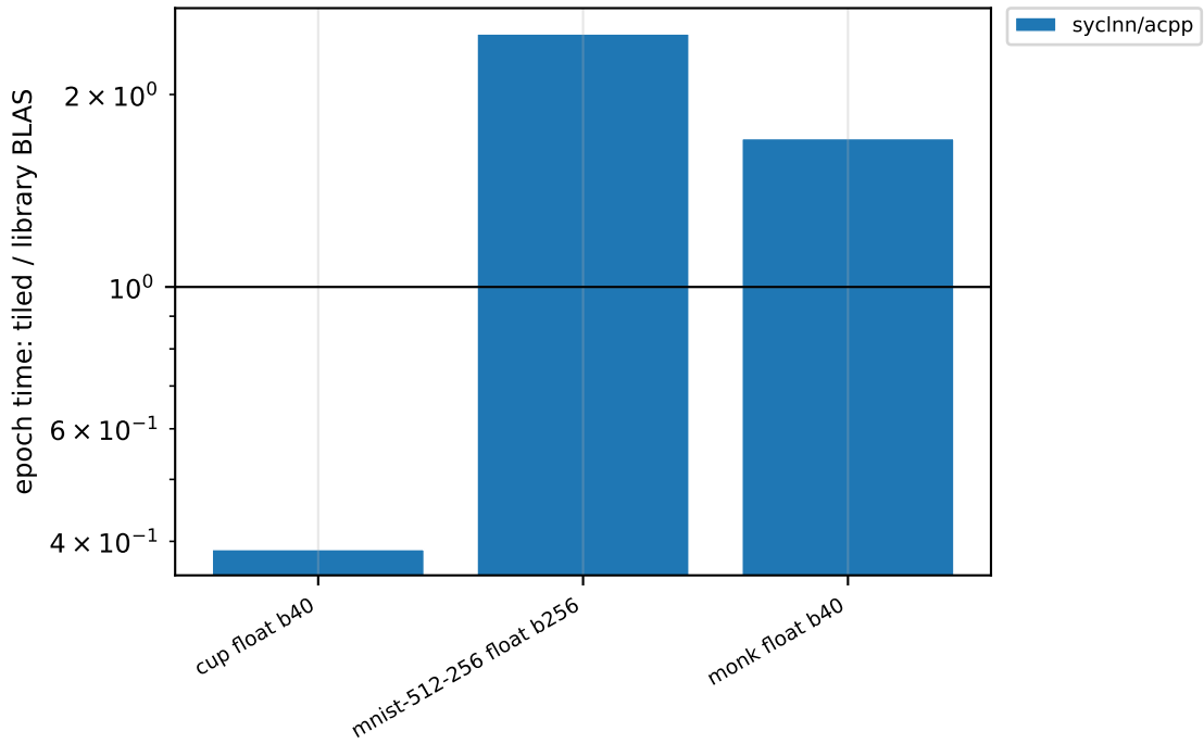
hand-written 16x16 tiled GEMM vs library on AdaptiveCpp OpenMP host device
