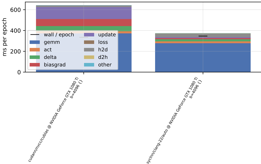
per-phase device time - sweep-w1024-d8-b4096 (float, train)
