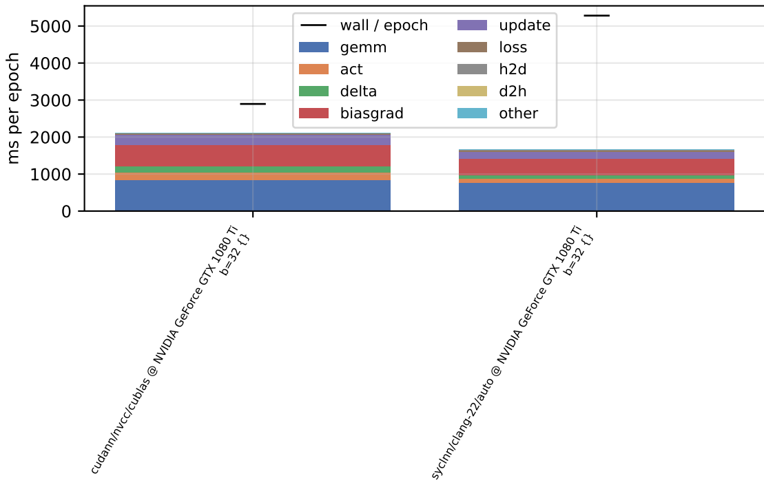
per-phase device time - sweep-w256-d8-b32 (float, train)
