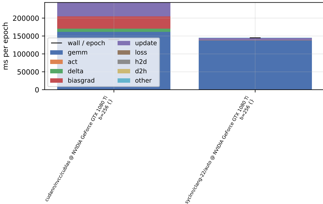
per-phase device time - sweep-w4096-d8-b256 (double, train)
