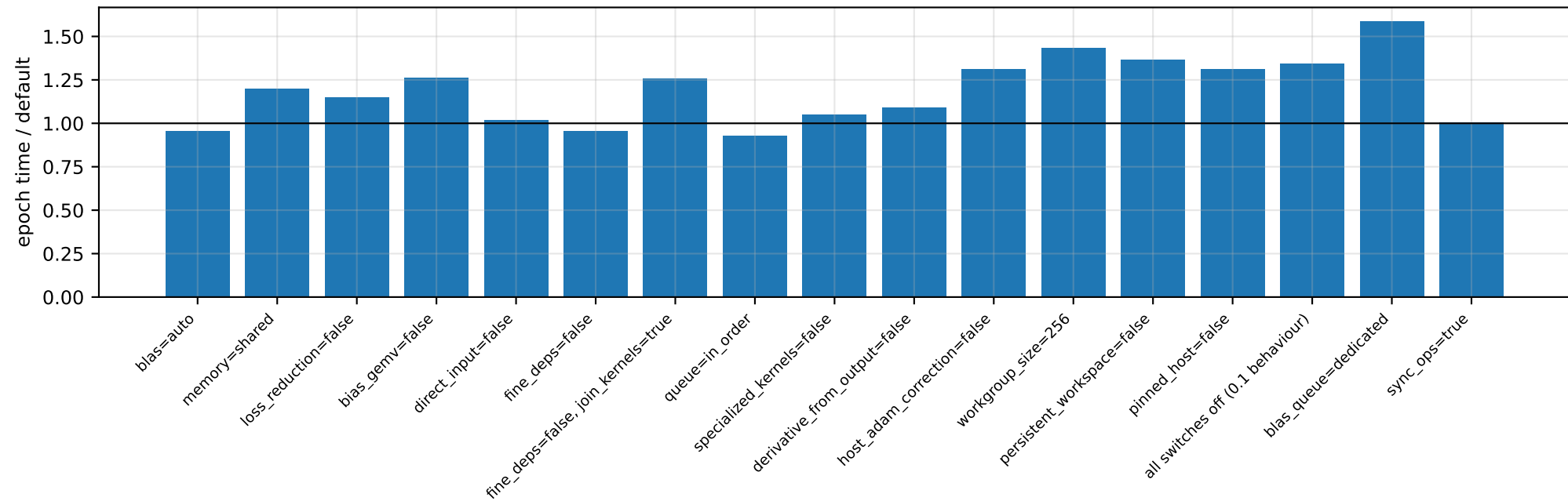
syclnn ablations - cup (float, b=40) on NVIDIA GeForce GTX 1080 Ti
