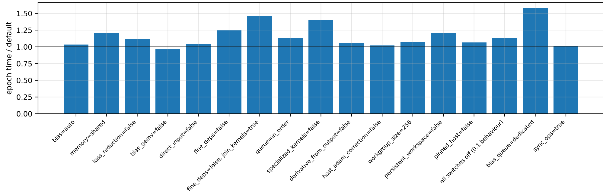
syncInn ablations - monk (float, b=40) on NVIDIA GeForce GTX 1080 Ti
