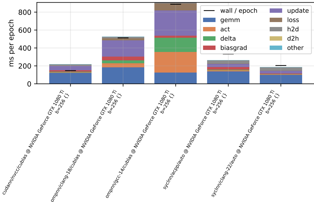
per-phase device time - mnist (float, train)
