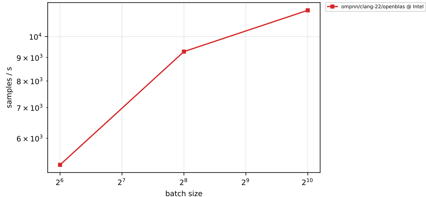
training throughput - mnist (double, cpu)
