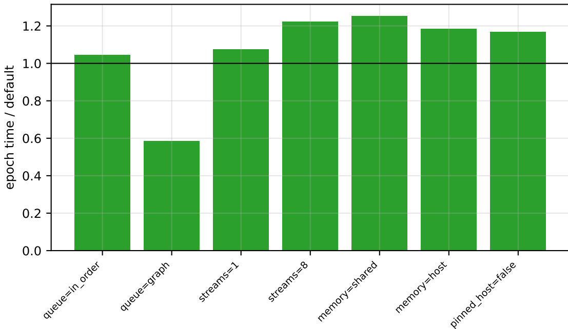
cudaann ablations - monk (float, b=40) on RX 7900 XTX
