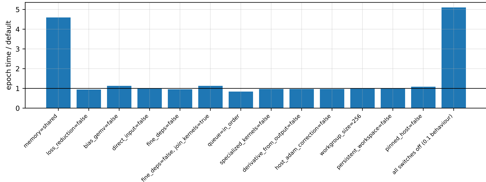
syclInn ablations - mnist-512-256 (float, b=256) on RX 7900 XTX
