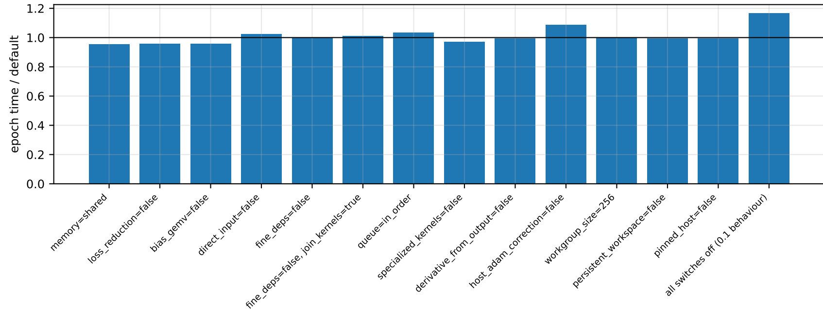
syclnn ablations - mnist-512-256 (float, b=256) on TR 2950X
