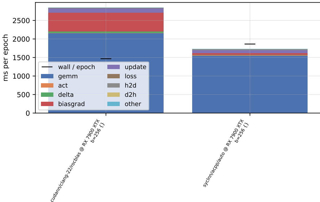
per-phase device time - sweep-w1024-d4-b256 (double, train)
