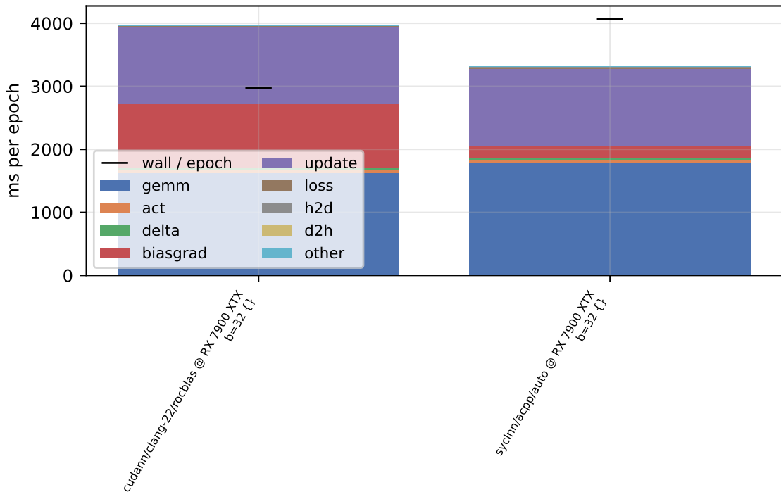
per-phase device time - sweep-w4096-d2-b32 (float, train)
