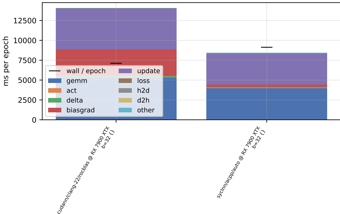
per-phase device time - sweep-w4096-d4-b32 (float, train)
