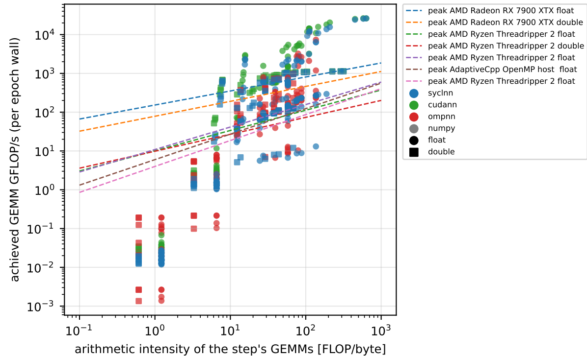
roofline placement of every training row
