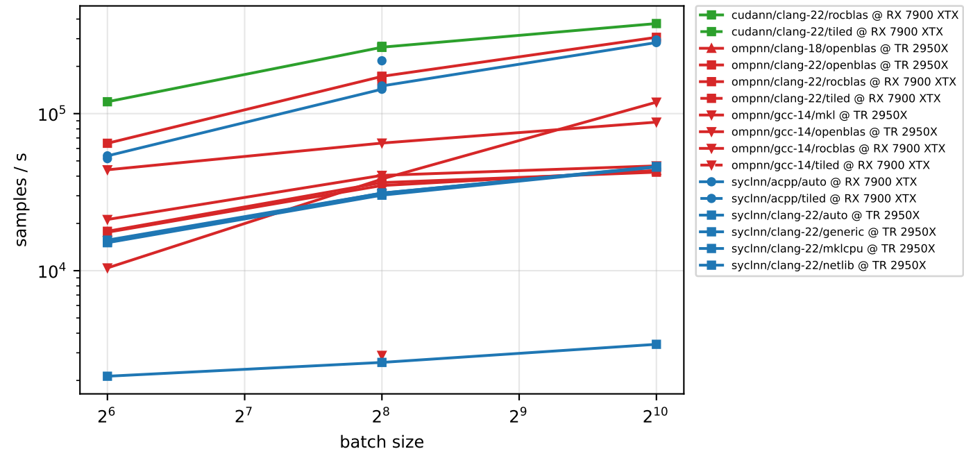
training throughput - mnist-512-256 (double)
