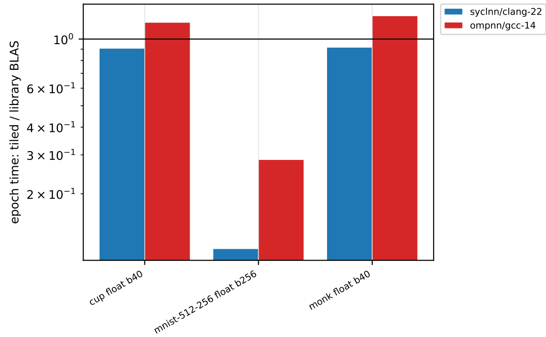
hand-written 16x16 tiled GEMM vs library on TR 2950X
