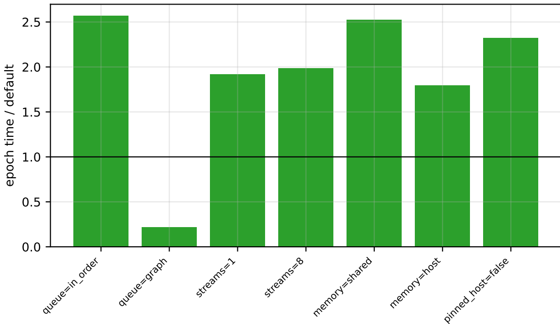
cudaann ablations - cup (float, b=40) on NVIDIA GeForce GTX 1080 Ti
