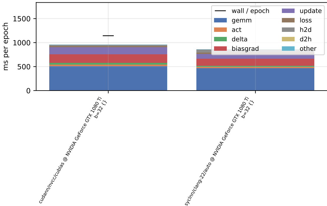
per-phase device time - sweep-w256-d2-b32 (double, train)
