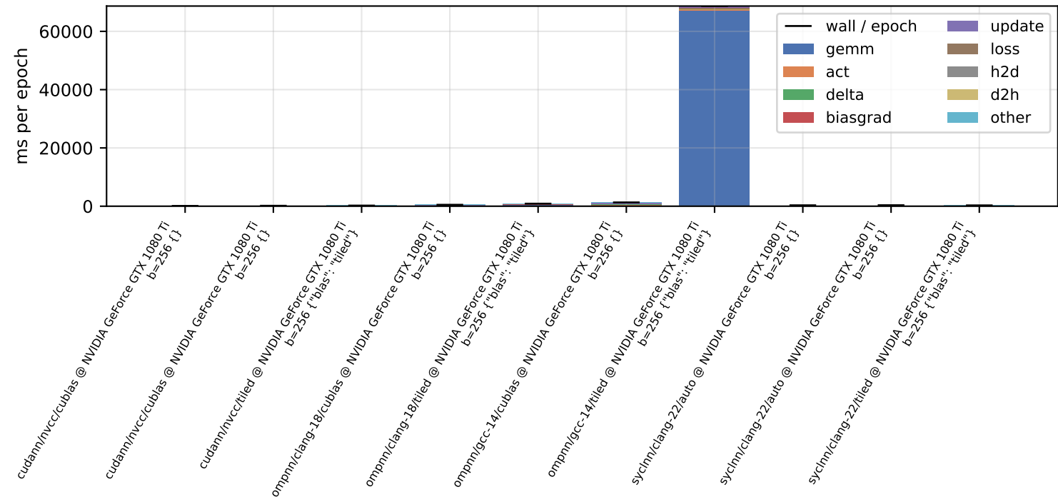
per-phase device time - sweep-w256-d4-b256 (float, train)
