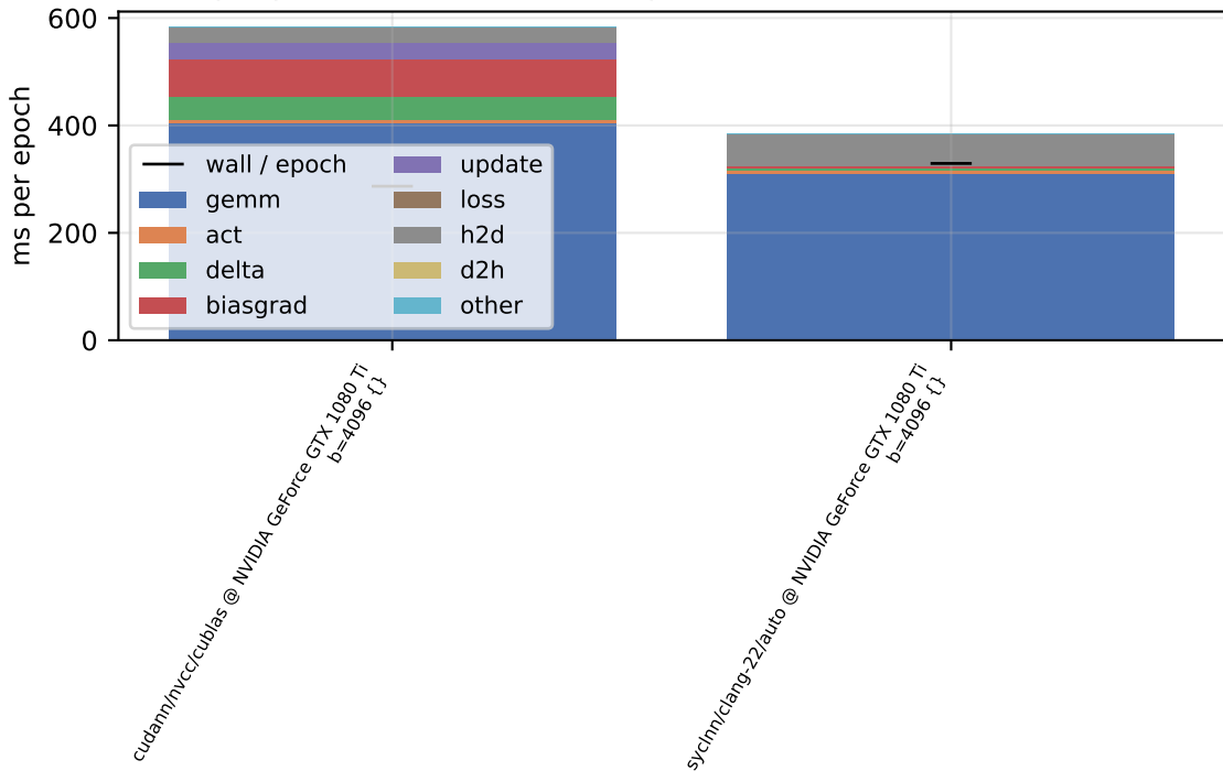
per-phase device time - sweep-w256-d4-b4096 (double, train)
