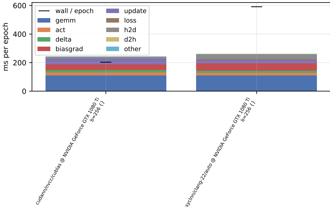
per-phase device time - sweep-w256-d8-b256 (float, train)
