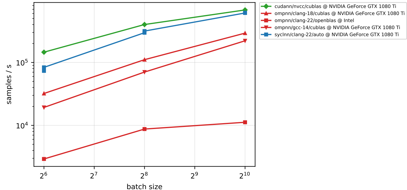
training throughput - mnist (float)
