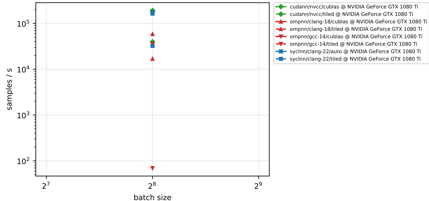
training throughput - sweep-w1024-d4-b256 (float)
