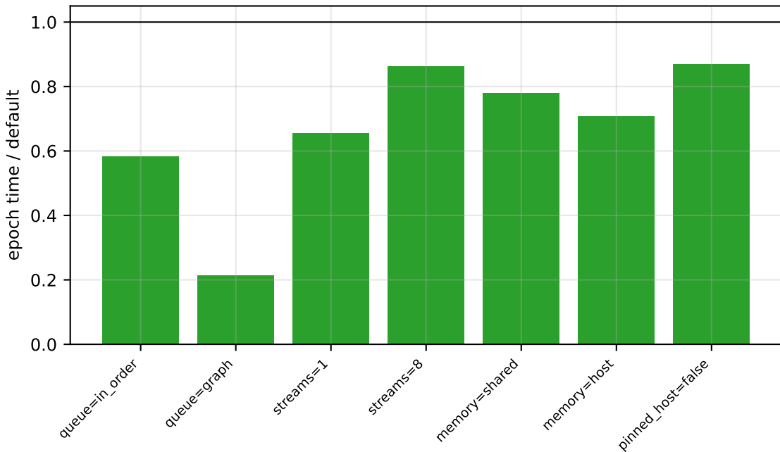
cudaNN ablations - cup (float, b=40) on RX 7900 XTX
