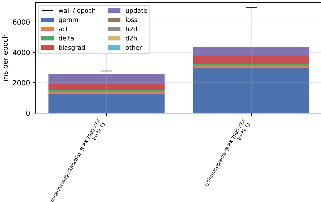
per-phase device time - sweep-w1024-d8-b32 (float, train)
