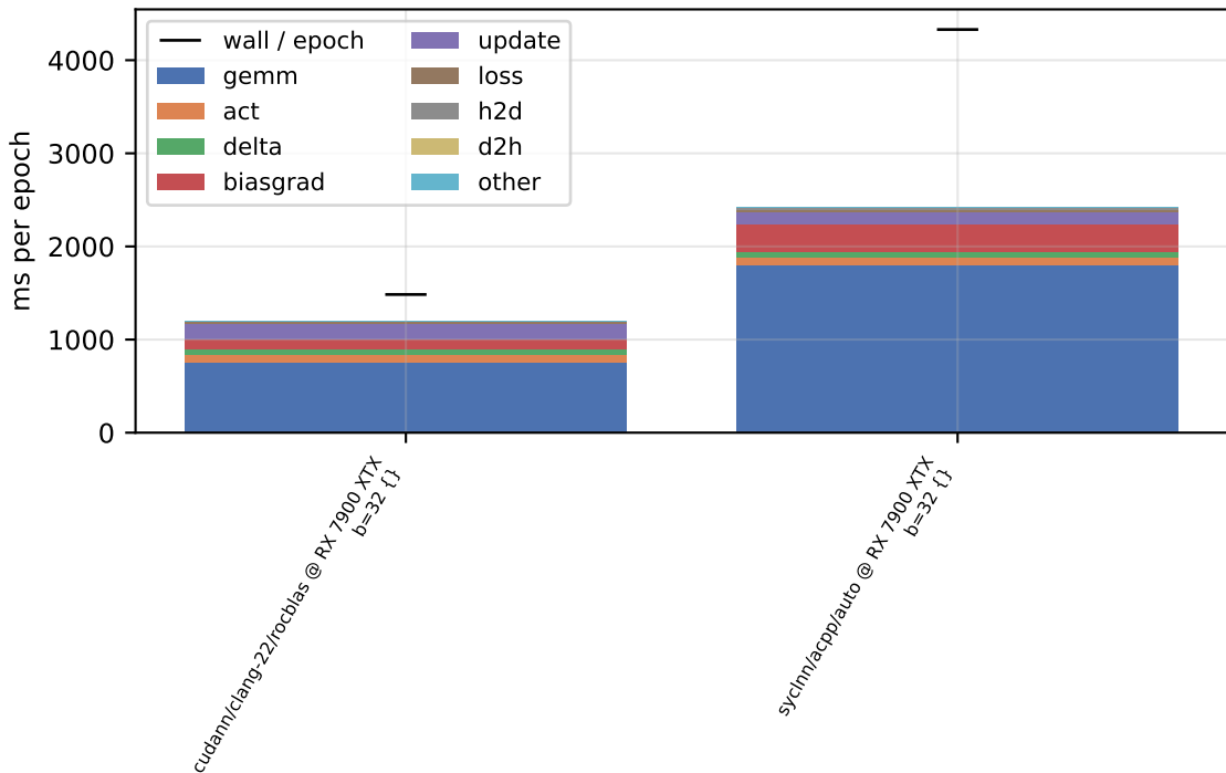
per-phase device time - sweep-w256-d4-b32 (double, train)
