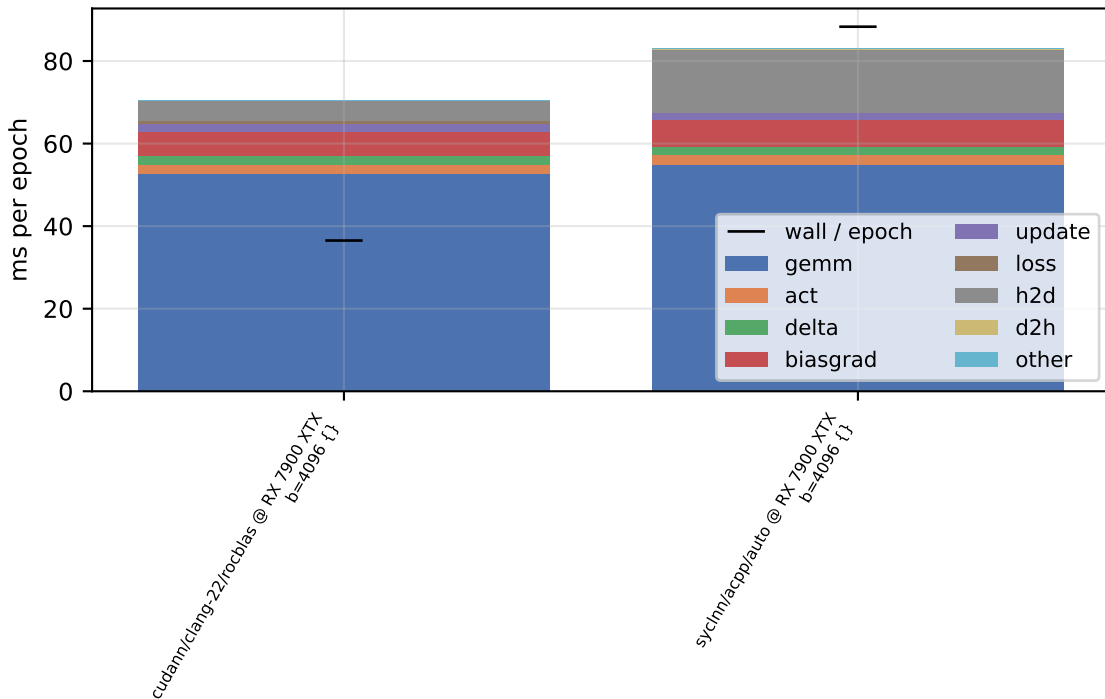
per-phase device time - sweep-w256-d8-b4096 (float, train)
