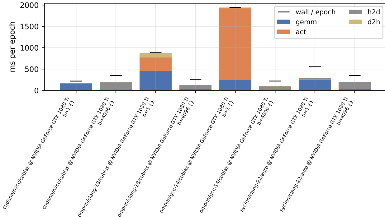
per-phase device time - mnist (float, infer)
