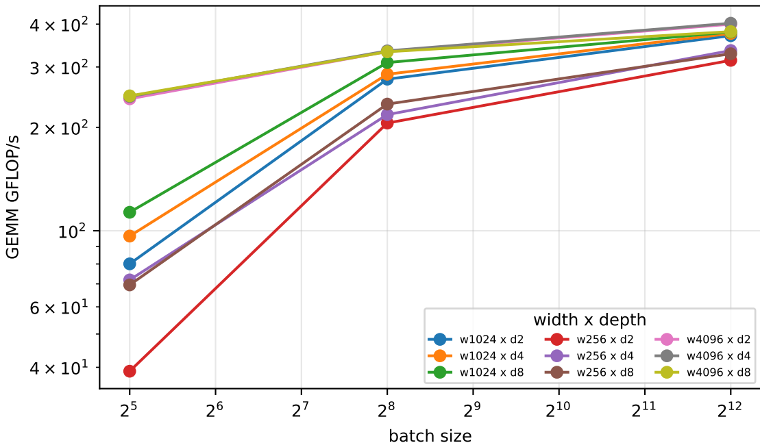
W4 sweep - cudann/nvcc/cublas @ NVIDIA GeForce GTX 1080 Ti (double)
