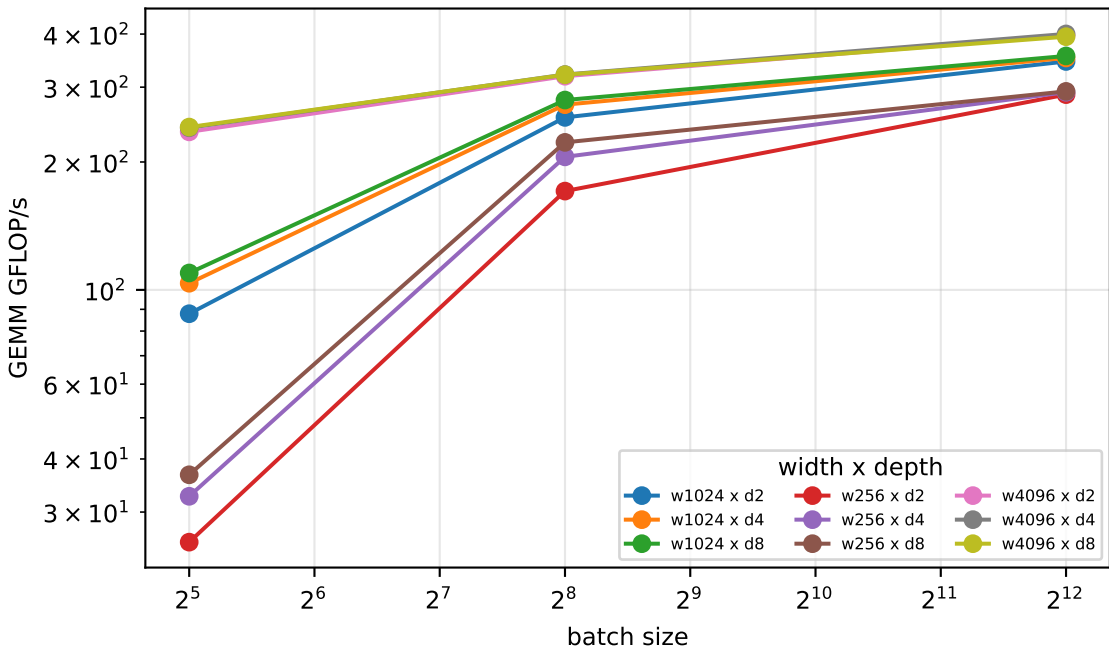
W4 sweep - syclnn/clang-22/auto @ NVIDIA GeForce GTX 1080 Ti (double)
