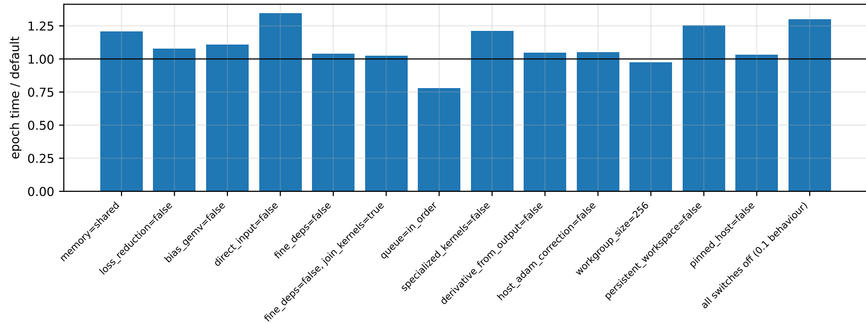
syclInn ablations - monk (float, b=40) on RX 7900 XTX
