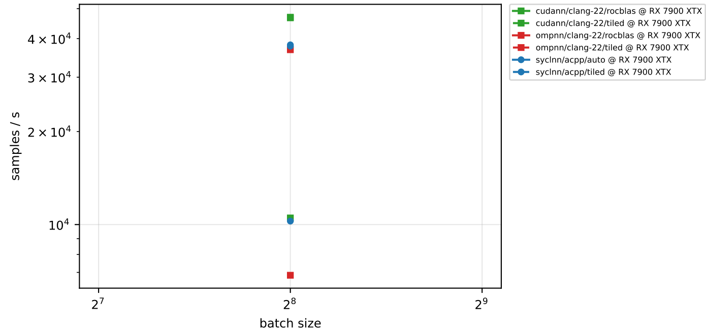
training throughput - sweep-w4096-d4-b256 (float)
