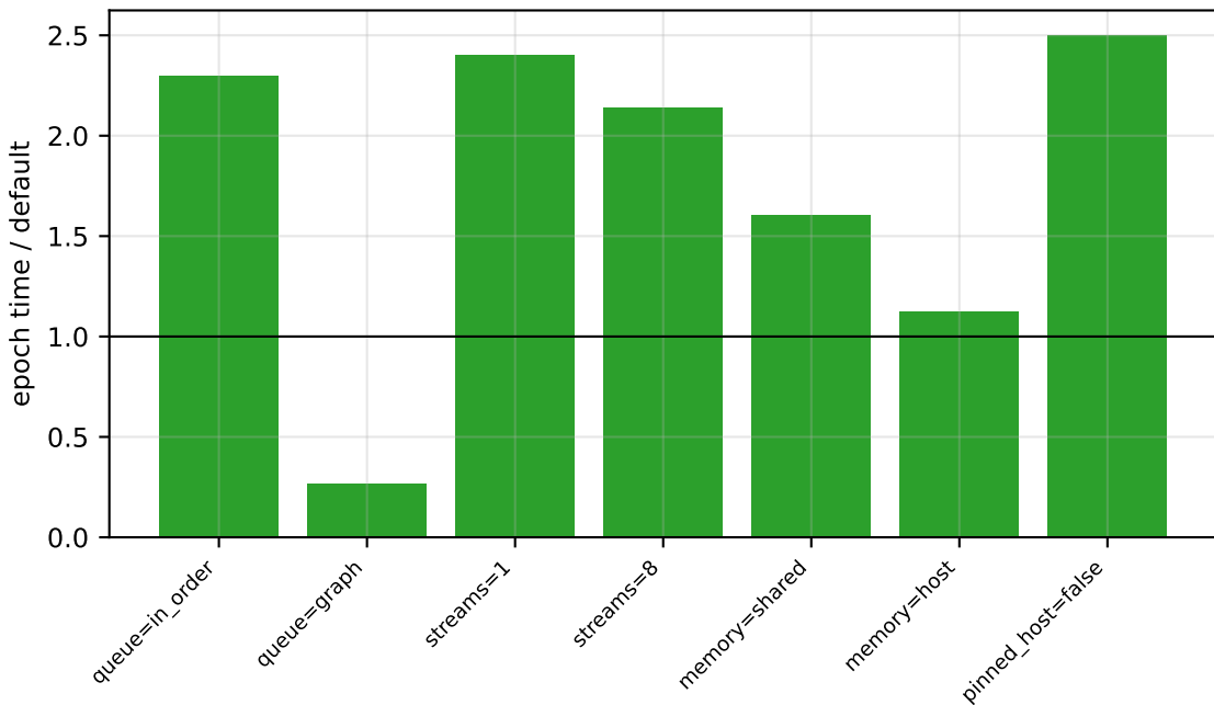
cudaann ablations - monk (float, b=40) on NVIDIA GeForce GTX 1080 Ti
