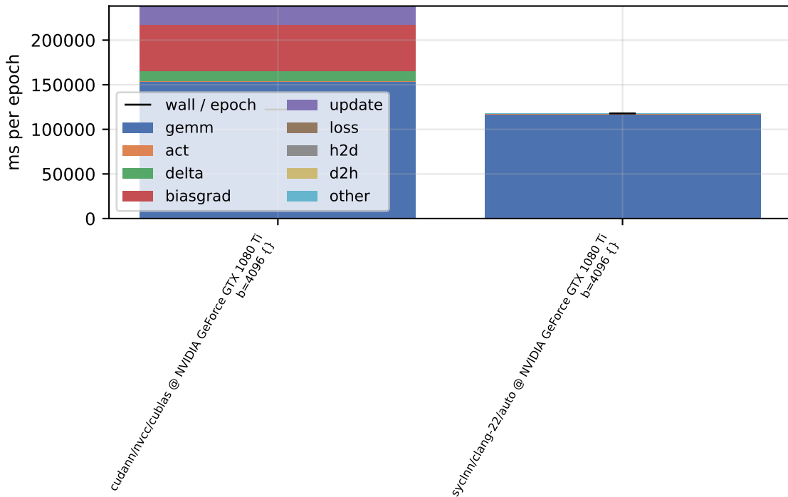
per-phase device time - sweep-w4096-d8-b4096 (double, train)
