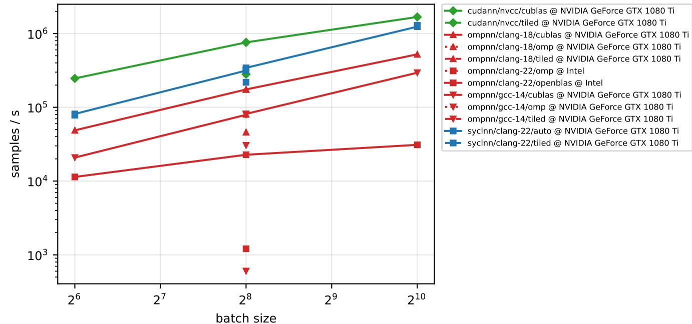
training throughput - mnist-512-256 (float)
