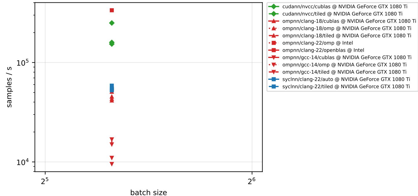
training throughput - monk (float)
