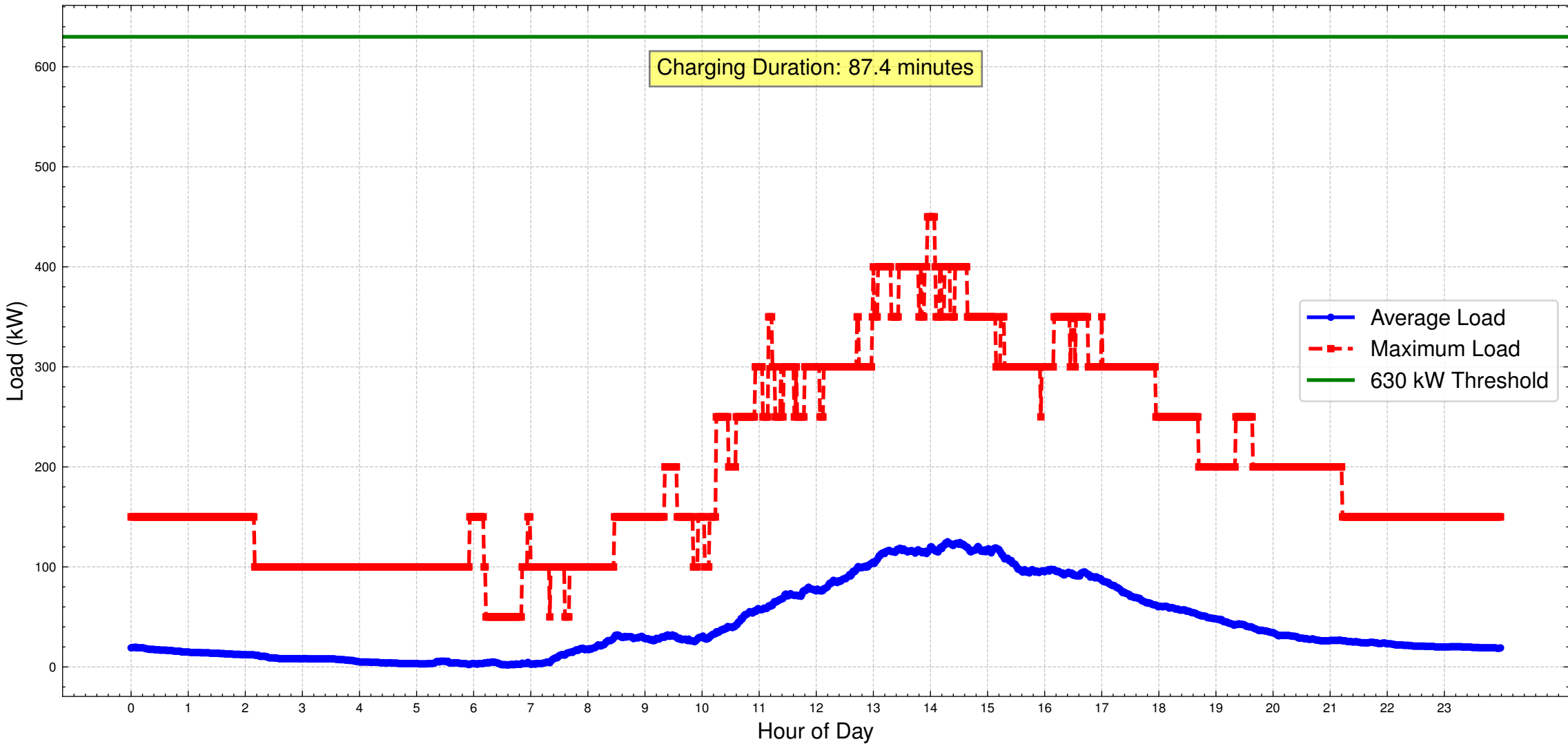
Daily Load Profile for Base 0 with 50 kW Charging (Active Days Only)
