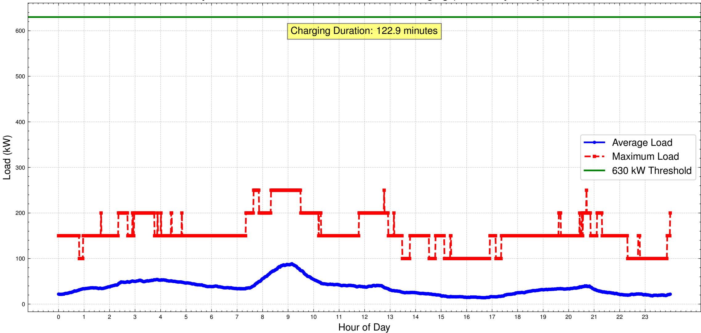
Daily Load Profile for Base 102 with 50 kW Charging (Active Days Only)
