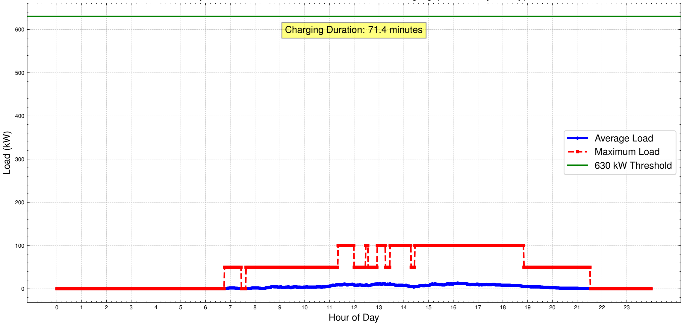
Daily Load Profile for Base 20 with 50 kW Charging (Active Days Only)
