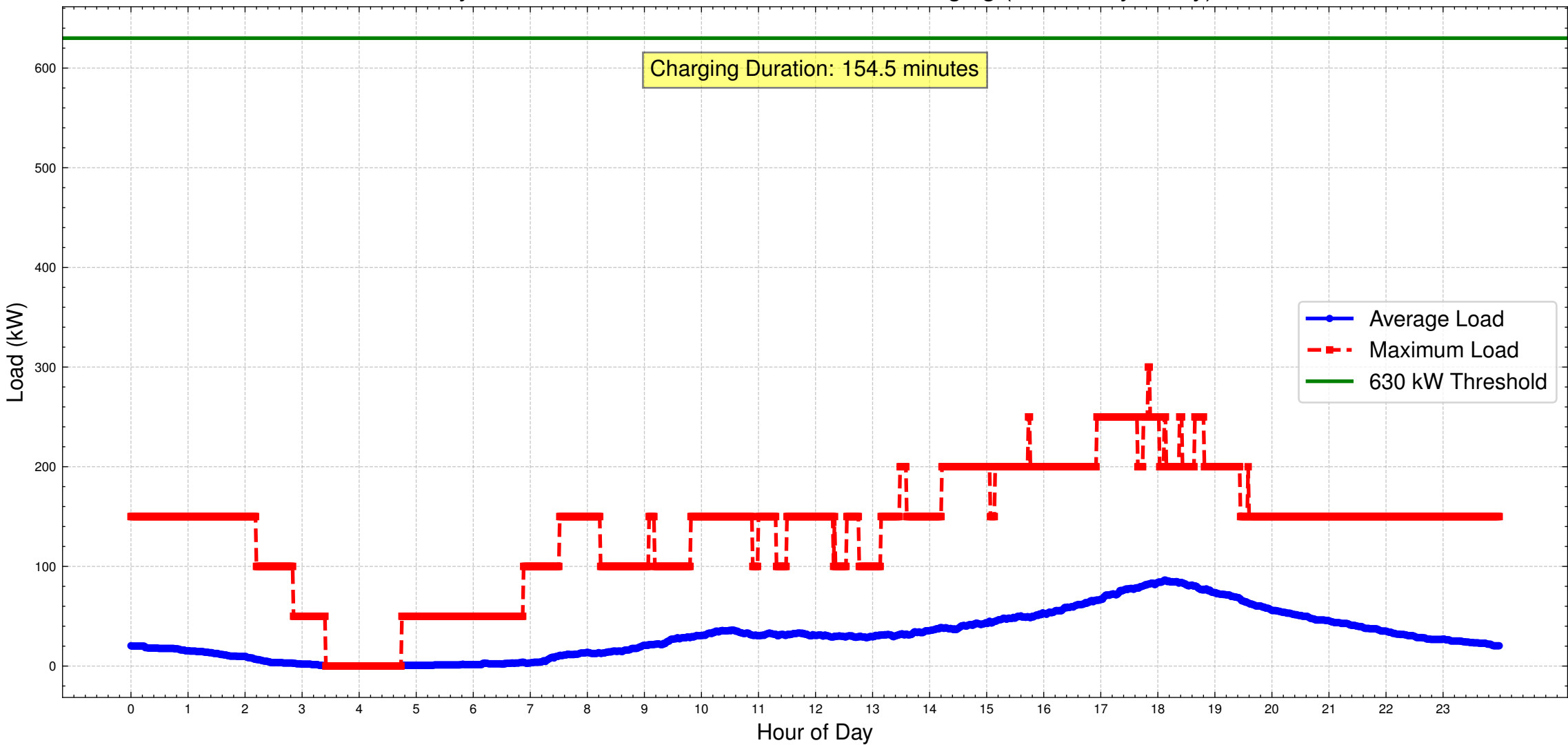
Daily Load Profile for Base 26 with 50 kW Charging (Active Days Only)
