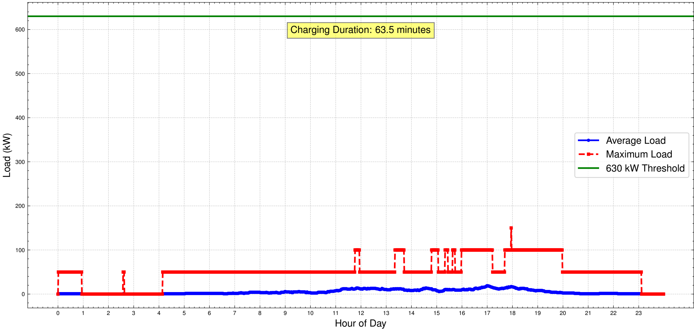
Daily Load Profile for Base 4 with 50 kW Charging (Active Days Only)
