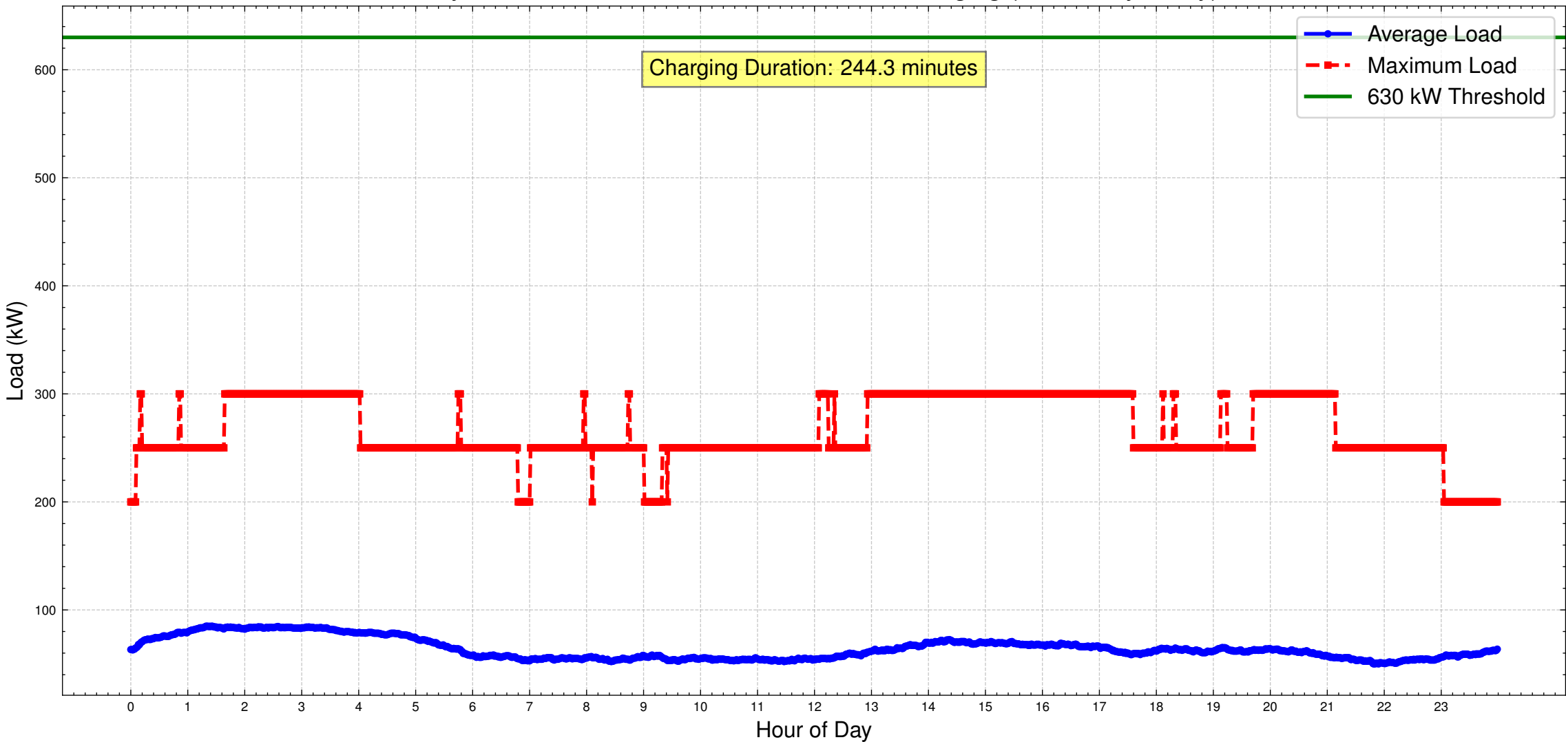
Daily Load Profile for Base 502 with 50 kW Charging (Active Days Only)
